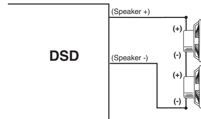
Two 8 Ohm Speakers
